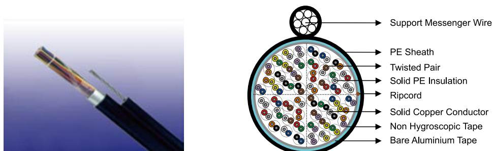
Fig 8 Solid PE Insulated & AP Sheathed (Alpeth) Air Core Cable to GR-421
